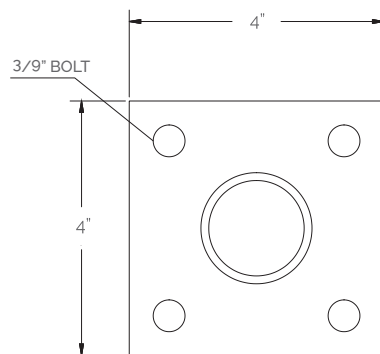
MOUNTING BRACKET
