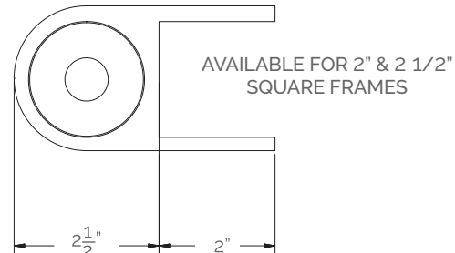
GATE MOUNT
